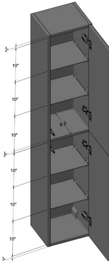
OPEN CABINET VIEW
