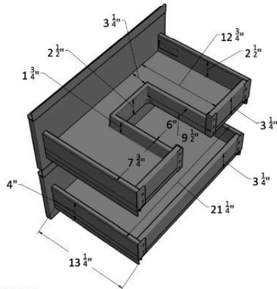
DRAWER SIZES
