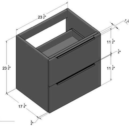
OUTSIDE SIZES
