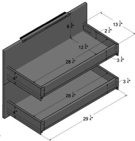
DRAWER SIZES
