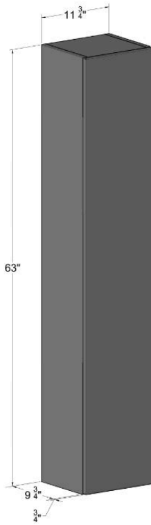
OUTSIDE SIZES
