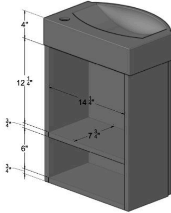
PLUMBING DETAIL SIZES
