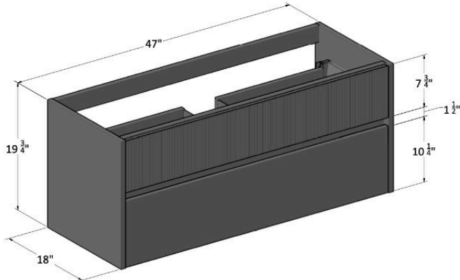
OUTSIDE SIZES
