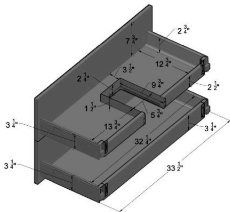
DRAWER SIZES
