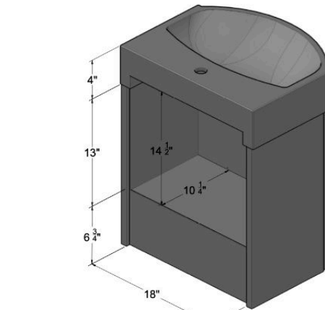
PLUMBING DETAIL SIZES
