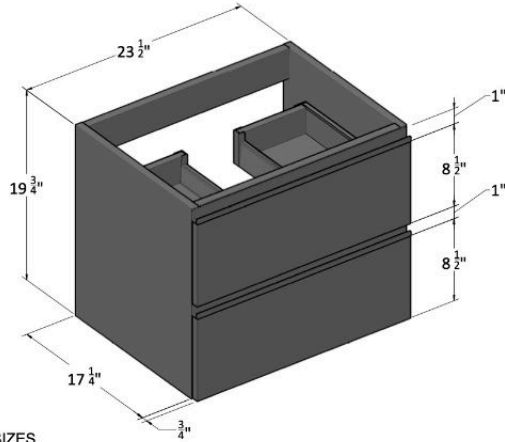
OUTSIDE SIZES
