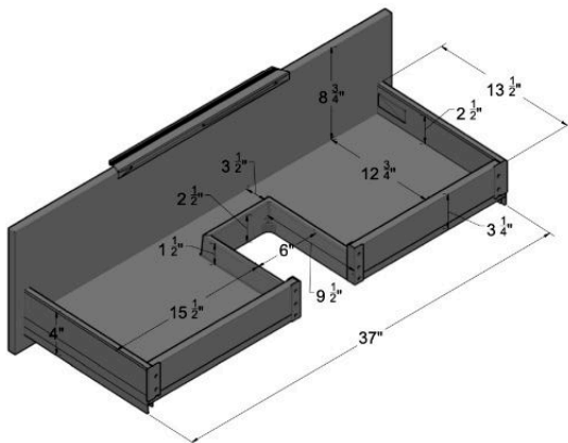
DRAWER SIZES
