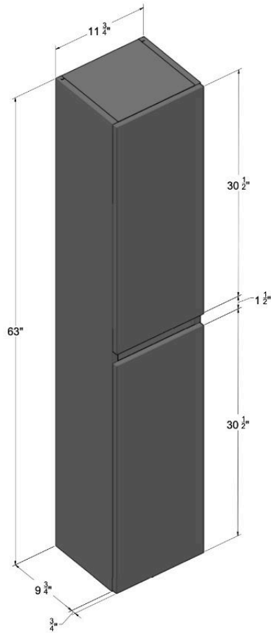
FRONT & SIDE VIEW
