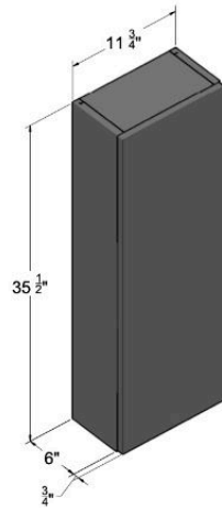
FRONT & SIDE VIEW
