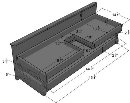
DRAWER SIZES
