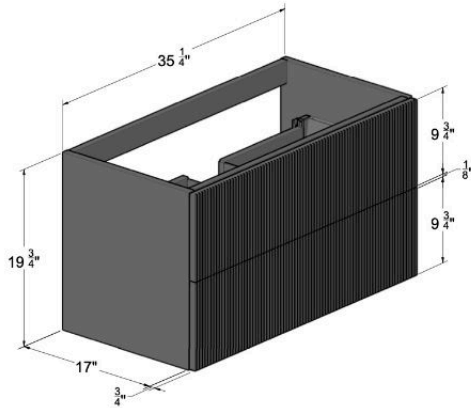
OUTSIDE SIZES
