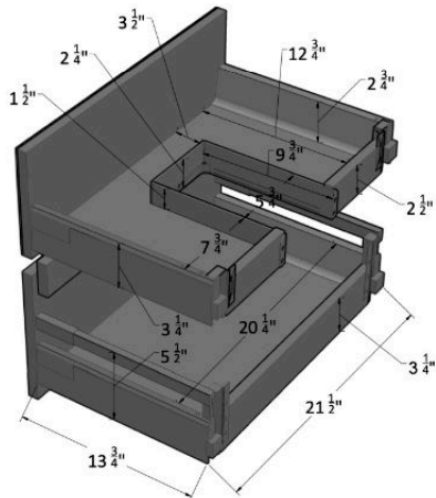
DRAWER SIZES
