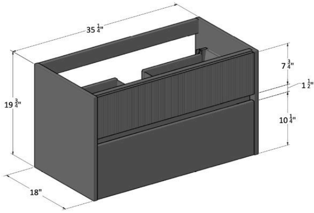
OUTSIDE SIZES
