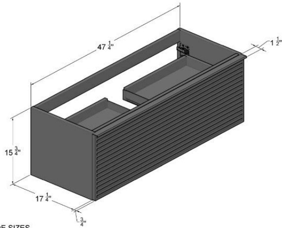
OUTSIDE SIZES
