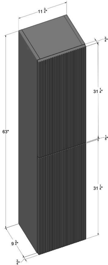
OUTSIDE SIZES
