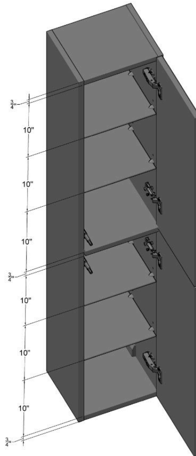
OPEN CABINET VIEW
