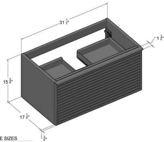
OUTSIDE SIZES
