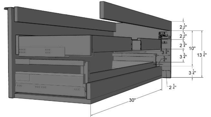
PLUMBING DETAIL SIZES
