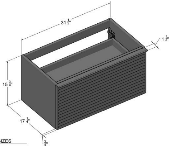
OPEN CABINET VIEW
