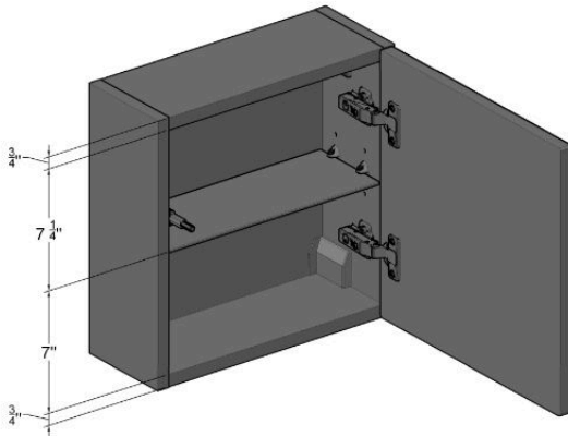
OPEN CABINET VIEW
