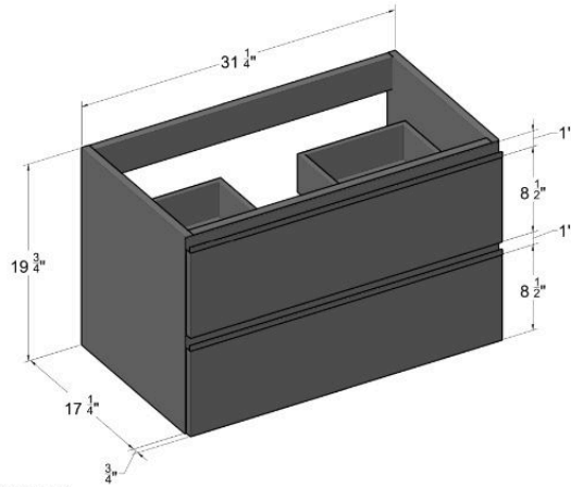
OUTSIDE SIZES
