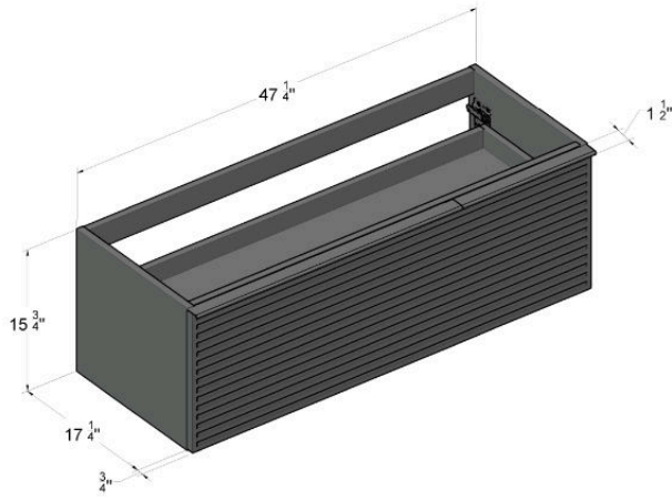
OUTSIDE SIZES
