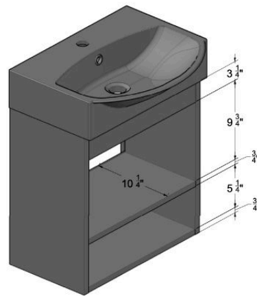
OPEN CABINET VIEW
