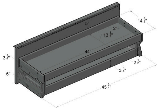
DRAWER SIZES
