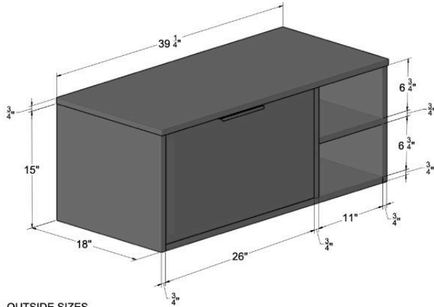
OUTSIDE SIZES
