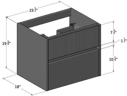
OUTSIDE SIZES
